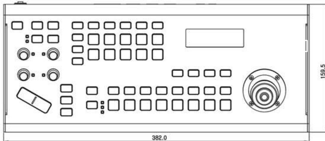
TOP View
